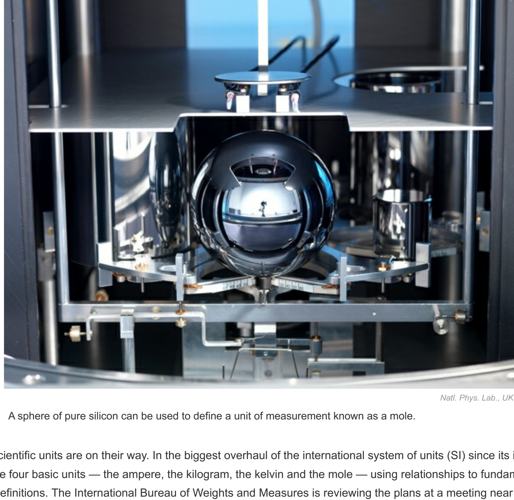
A sphere of pure silicon can be used to define a unit of measurement known as a mole.
