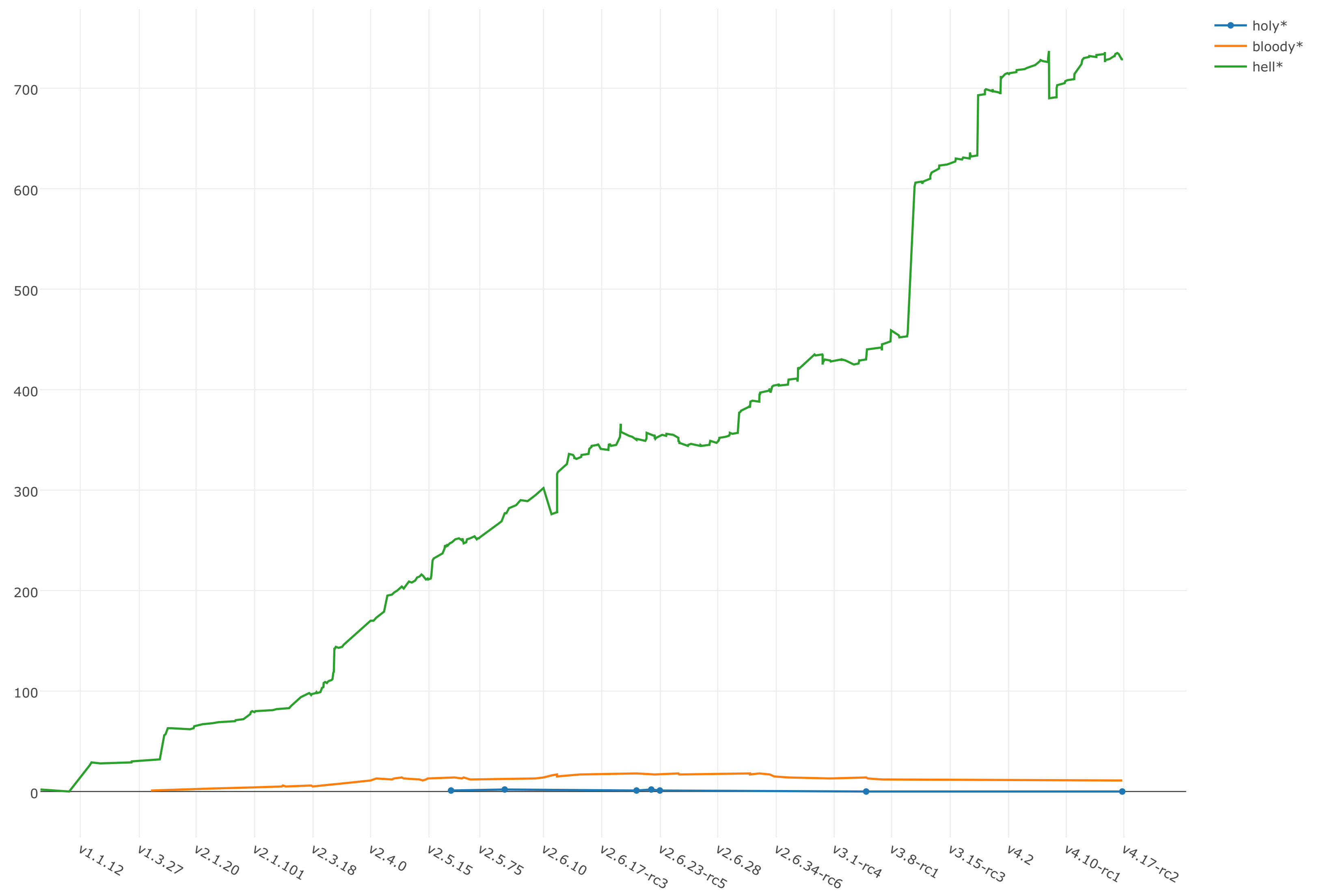
Occurrences of words in the Linux kernel source code over time
